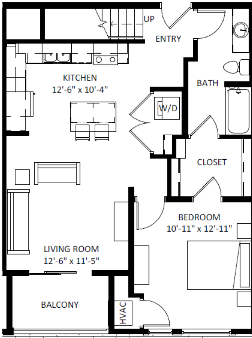
FIRST FLOOR
